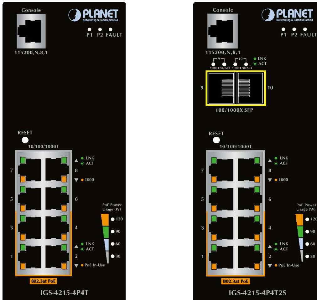
Figure 2-1-2a IGS-4215-4P4T and IGS-4215-4P4T2S Front Panel
