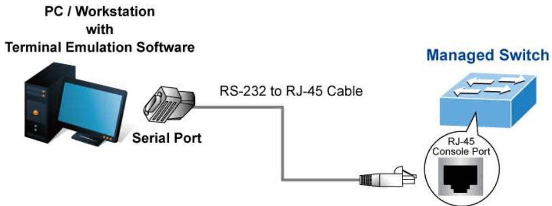
Figure 3-1-1: Console Management
