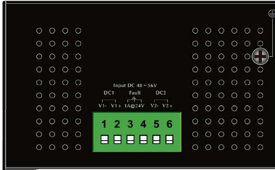
Figure 2-1-4a: Industrial Gigabit PoE Switch Upper Panel.
