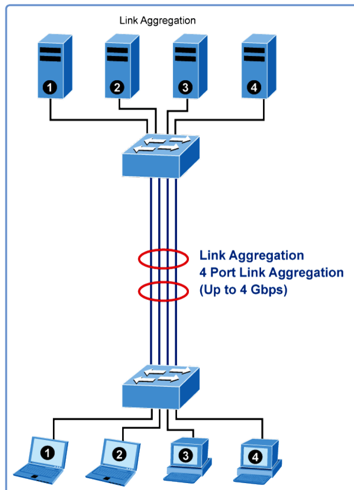
Figure 4-4-1 Link Aggregation
