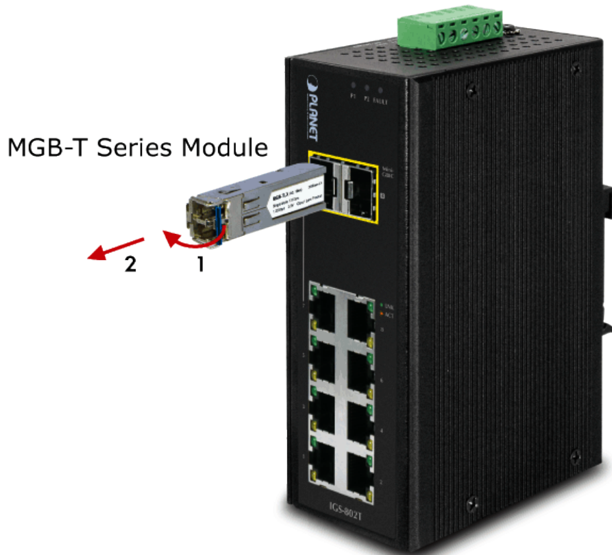
Figure 2-10: Pull out the SFP Transceiver Module
