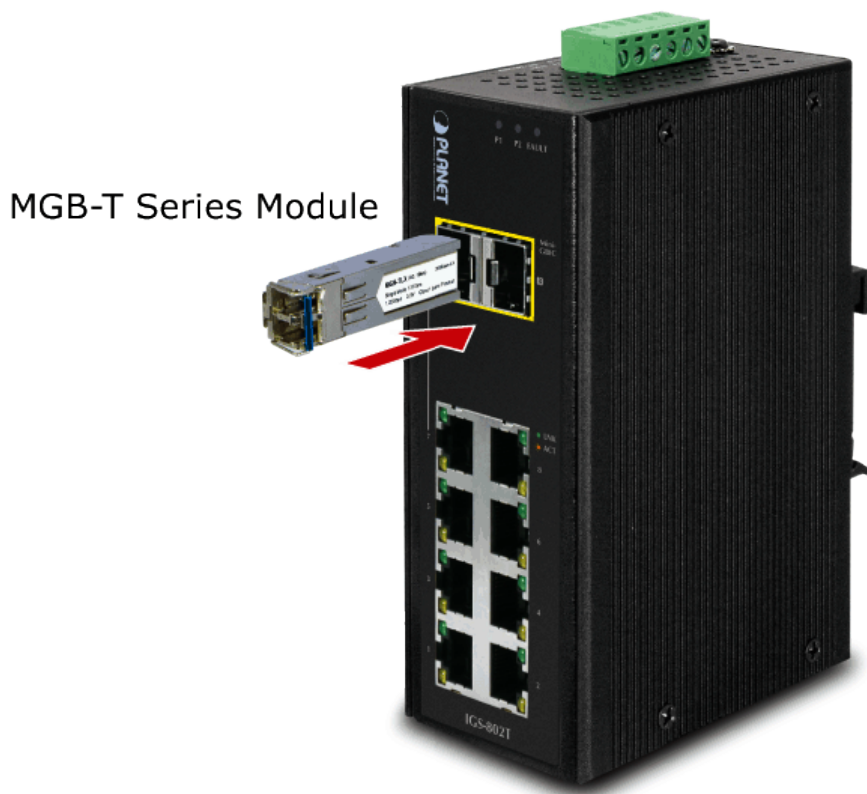
Figure 2-2-4a: Plug in the SFP Transceiver
