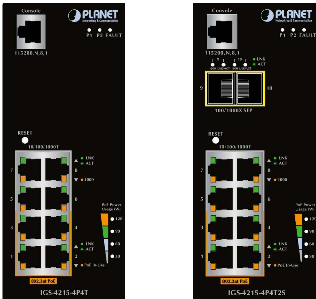
Figure 2-1-3a IGS-4215-4P4T and IGS-4215-4P4T2S LED Panel
