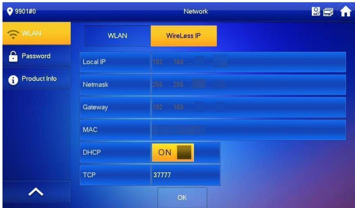
Figure 2-43 Wireless IP
