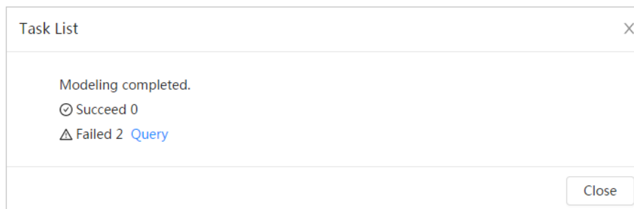
Figure 8-13 Modeling result
